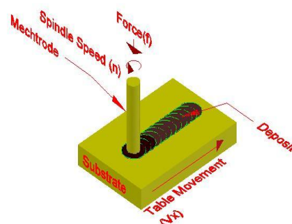
Figure 1: Schematic representation of friction surfacing process.
